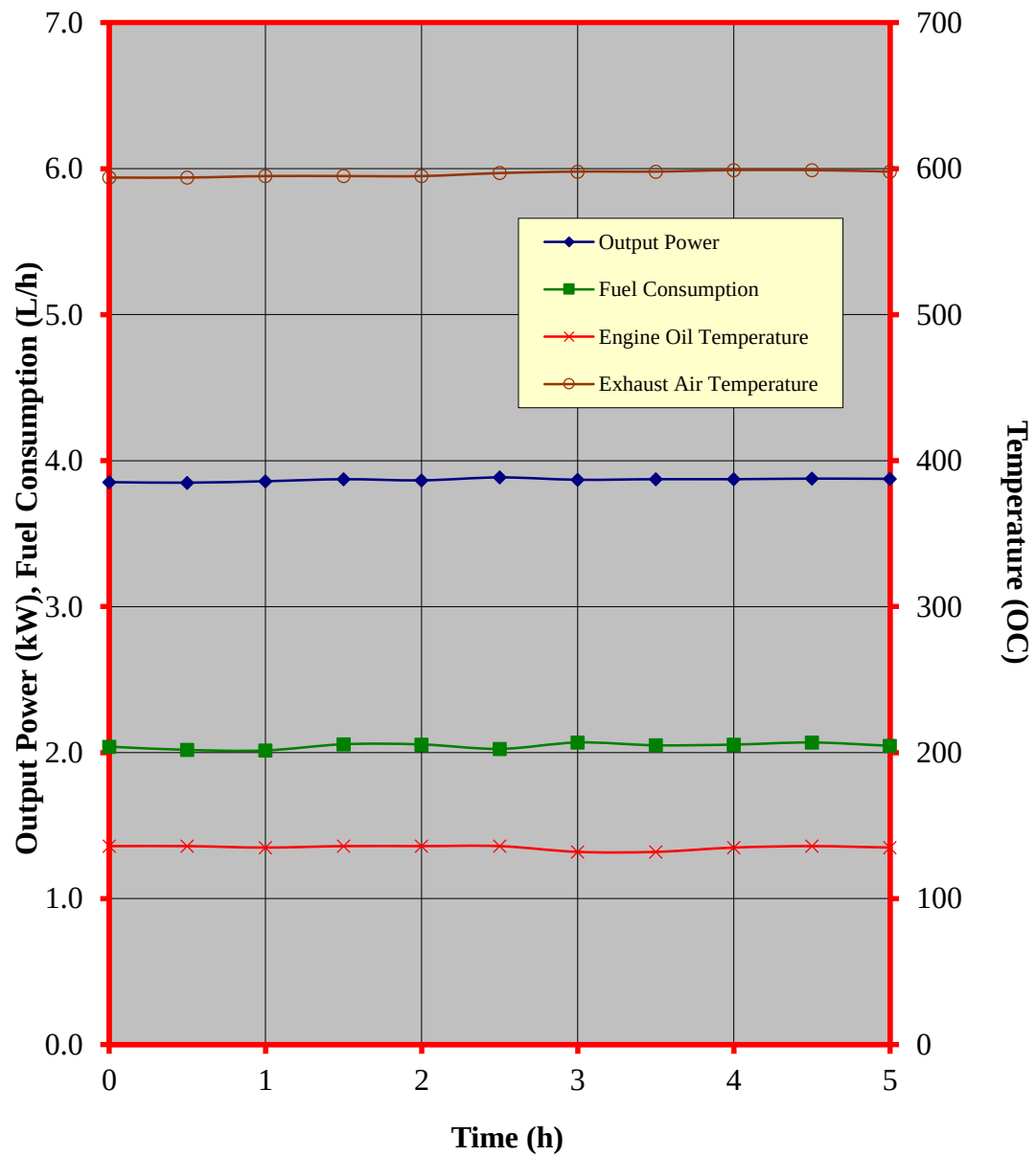
Figure 4. Performance characteristic curves during the continuous running test of the HONDA GX200H LHB2 gasoline engine
