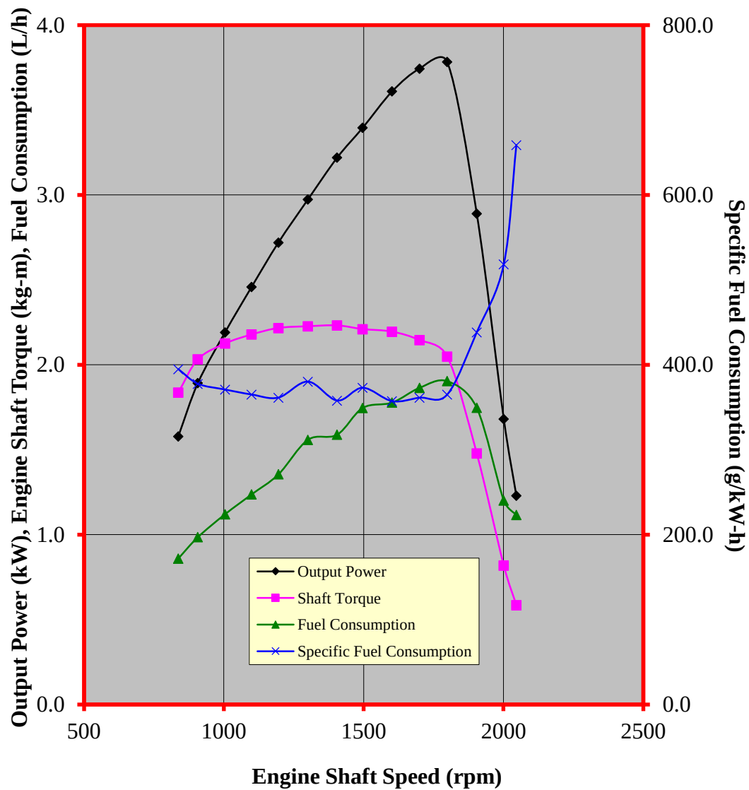
Figure 3. Performance characteristic curves of the HONDA GX200H LHB2 gasoline engine
